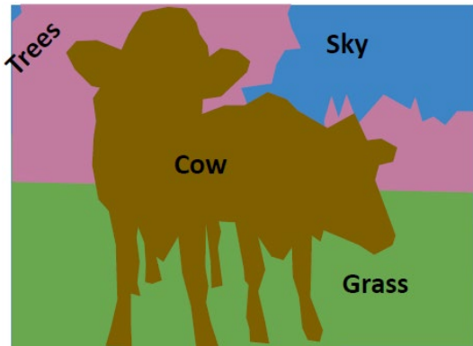
Semantic Segmentation
