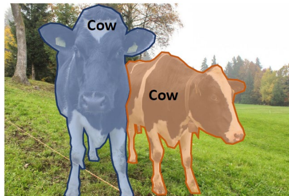
Instance Segmentation
