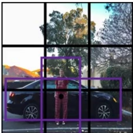
Anchor box 1:
